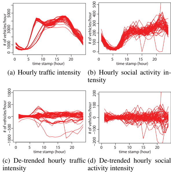
Figure 1: Data de-trending
