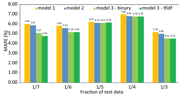
(a) MAPE
