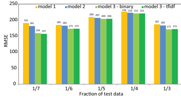
(b) RMSE
