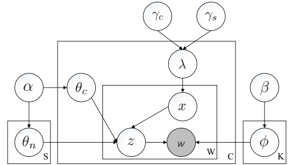
Figure 2: Graphical representation of DCT model.
