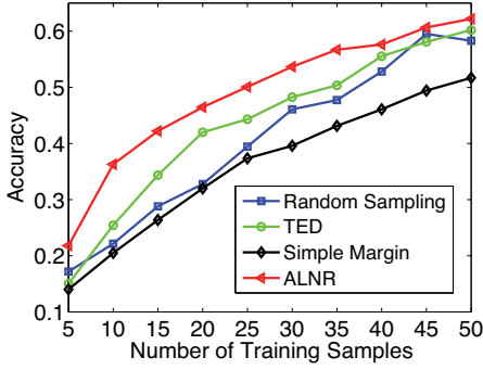
Figure 4: The average classification accuracy versus the number of training samples.
