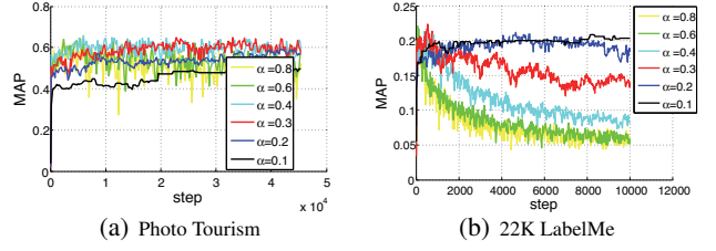
Figure 6: Effect of similarity threshold \alpha .
