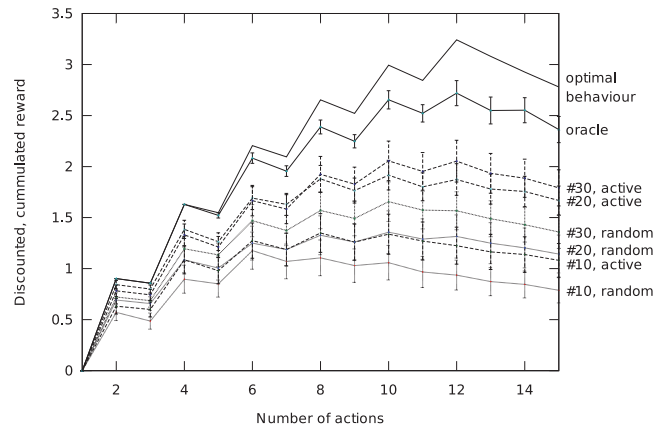
Figure 5: Experiment 3: Full relational reinforcement learning scenario. The performance is measured as mean discounted reward. Each curve is annotated with the method used to ground the symbol and the number of queries where applicable. The active learner requires significantly fewer samples to learn grounded relational symbols which permit an autonomous agent to plan for high-reward states.
