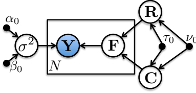
Figure 1: Graphical illustration of BFCM.
