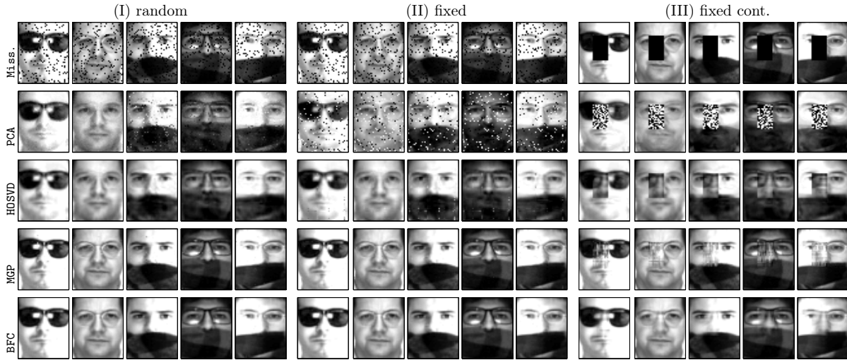
Figure 4: Predict missing pixels in face images. (I) missing at random positions in each image, (II) missing at fix positions in all images, (III) missing at a fixed and contiguous rectangle in all images. The top row shows example images with missing pixels. The 2nd to the 5th rows shows predicted images by different probabilistic models: PCA, HOSVD, Matrix Gaussian process (MGP) and BFCM. Note: for prediction task (II) and (III), the 2D-array structure of data must be accounted for, because the missing pixels are unseen in all images.
