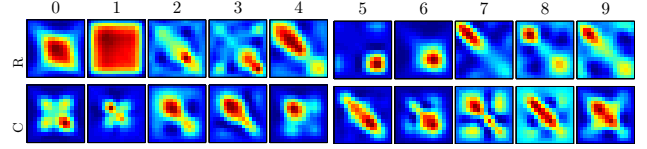
Figure 2: Row/column covariance of hand-written digits.
