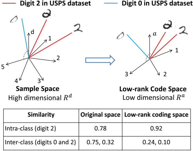
Figure 1: Similarity metrics in the original space and low-rank code space.
