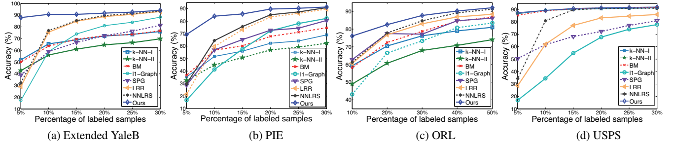
Figure 3: Accuracy of our approach and compared methods versus different percentages of labeled samples on four databases.
