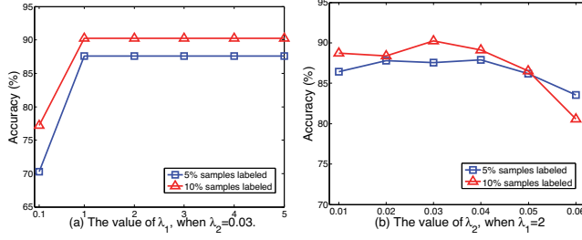
Figure 2: Accuracies of our graph under different values of (a) \lambda_1 and (b) \lambda_2 on extended YaleB face database.
