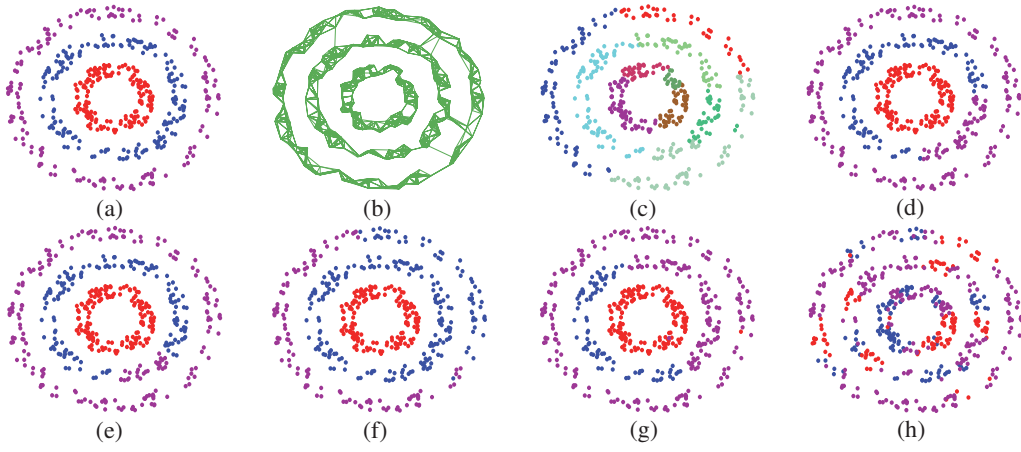
Figure 1: Toy example on the synthetic data set Syn-1K. Top 4 figures, from left to right: (a) ground-truth partition; (b) k-NN graph; (c) initial clustering results by shortest path, when d = 10 ; (d) clustering results by ESCG. Bottom 4 figures, from left to right: clustering results by (e) ESCG-R after 5 iterations; (f) spectral clustering; (g) RESC; (h) Nyström method.
