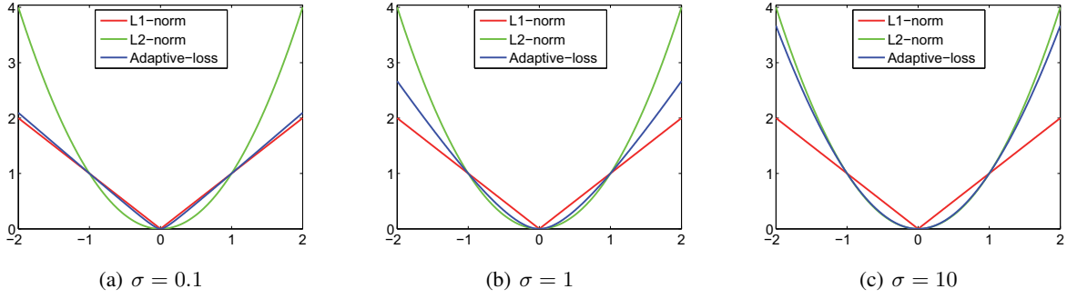
Figure 1: Illustration of L1-norm, L2-norm and the adaptive Loss function with different \sigma .
