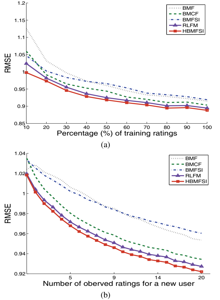
Figure 2: RMSE on MovieLens-100k data in cold-start situation: (a) hold-out prediction case, (b) fold-in prediction.
