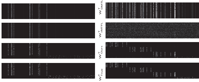
Figure 1: Comparison of the learned coefficient matrices using various MTL algorithms with the ground truth matrix. For each matrix, the rows correspond to tasks and the columns represent feature dimensions. We consider two scenarios, a major task group peppered with outlier tasks ( left ), and multiple groups of major tasks peppered with outlier tasks ( right ). This figure is best viewed on screen with magnification.
