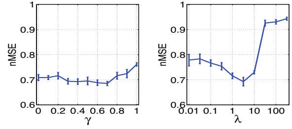
Figure 2: Performance of MTL-IRLS on the School dataset using various parameters ( \gamma and \lambda ).
