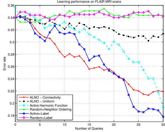
(a) Error rate on FLAIR scans
