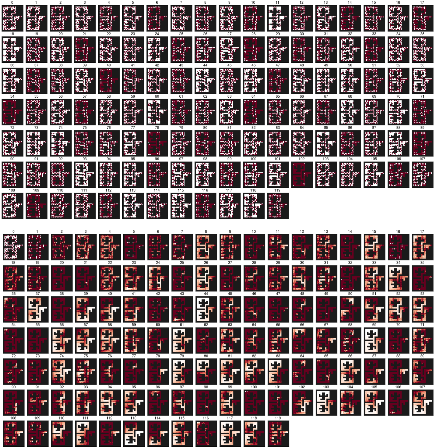
Figure 4: Each of the 120 images shows the value of a given feature for each state in the 7-room grid world, as produced by PSR tests (top) and forecasts (bottom). Walls are black, and feature values are color coded on a normalized scale from red (maximum) to white (minimum). Each is labeled with an index indicating in which order the feature was generated. Note how many forecasts appear to encode interesting properties of the environment: forecast 8 locates the markers; 38 identifies the dead-end corridor (where the goal will be hidden); 50 reveals a high-level symmetry based on multiple rooms (the upper 3 are a rotated version of the lower 3); 61, corridor crossings; 69, distance to the dead end; 76, non-room corridors that connect rooms; 88, a room that is not in a group of 3; 100, furthest point from the dead end, etc.
