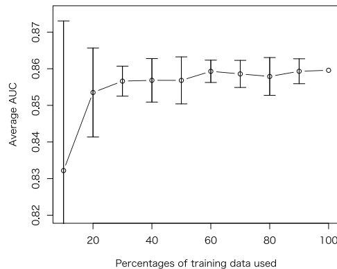
Figure 5: Average AUC for different amount of training data.
