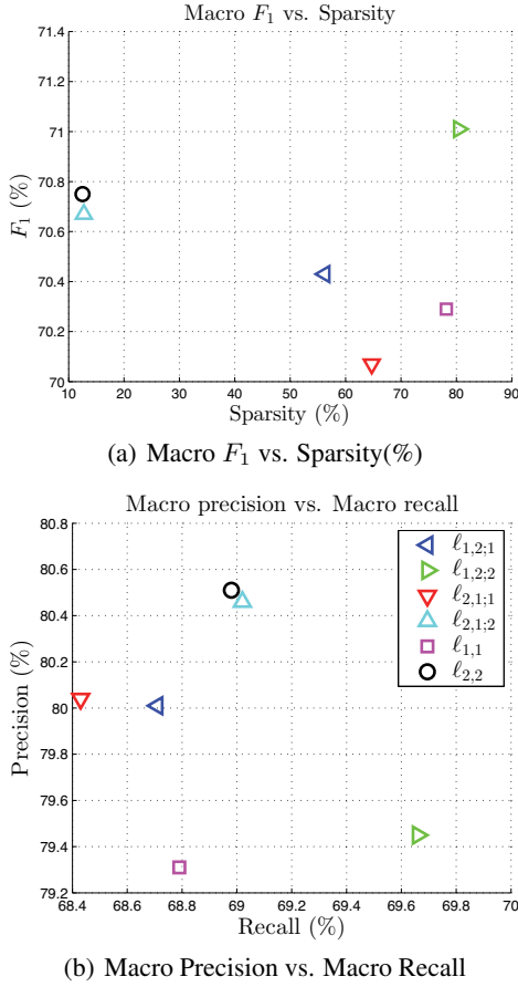
Figure 1: Summary of performance results on 14 multi class tasks
