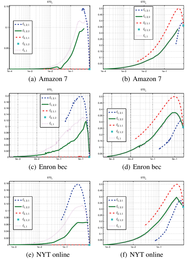
Figure 2: Group sparsity STD vs fraction of non-zero elements (log scale). Left: Feature sparsity STD. Right: Class sparsity STD.
