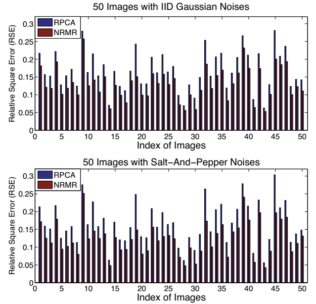
Figure 2: Results on the 50 test images, each contaminated with i.i.d. Gaussian noises or salt-pepper noises. On average, RPCA conducts 39.0 times SVD, while NRMR conducts 72.5 times SVD.
