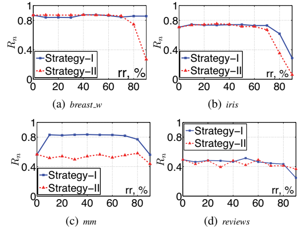
Figure 2: Performances of KCC on Incomplete BPs
