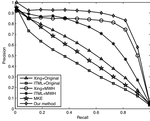
Figure 2: Precision-recall curve for image retrieval on NUS-WIDE-1.5K dataset
