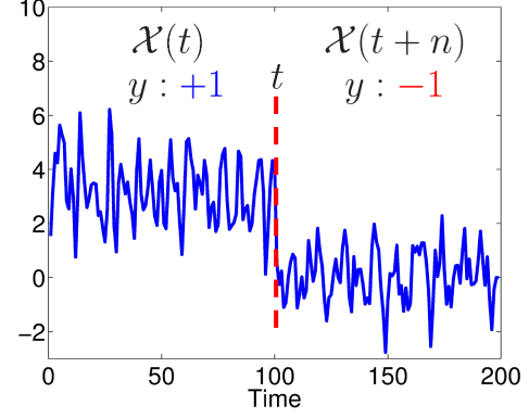
Figure 1: Illustrative example of two intervals \mathcal{X}(t) and \mathcal{X}(t+n) for 1D time series.
