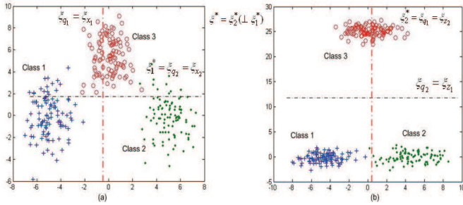
Figure 2: An example illustrating that the algorithm fails on SynSet2. (a) In the first view, Q and M_x disagree with each other, and the solution direction for view 1 is \xi_1^* = \xi_{q2} = \xi_{x2} . (b) In the second view, Q and M_z agree with each other on the direction \xi_2^* = \xi_{q1} = \xi_{z2} . In this case, the two views disagree with each other. The algorithm selects \xi^* = \xi_2^*(\perp \xi_1^*) as the final solution direction, which however is not correct.
