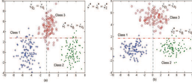
Figure 1: An example illustrating that the algorithm works properly on SynSet1. (a) In the first view, both Q and M_x agree with each other on the direction \xi_1^* = \xi_{q1} = \xi_{x2} . (b) In the second view, Q and M_z disagree with each other, and the solution direction for view 2 is \xi_2^* = \xi_{q1} = \xi_{z1} . Since the two views agree with each other, the final solution direction is \xi^* = \xi_1^* = \xi_2^* , which is optimal.
