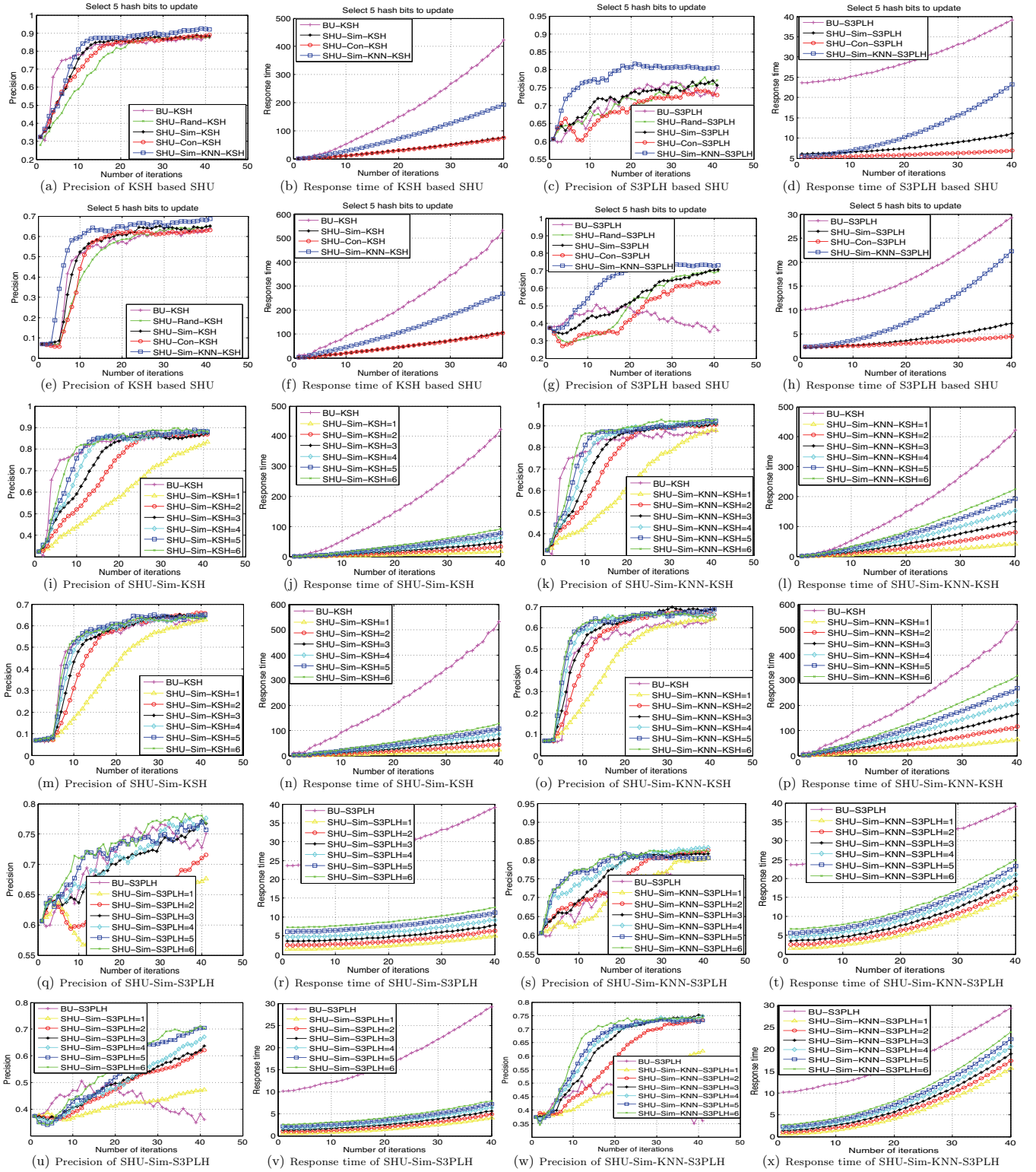
Figure 2: Precision (@top 500) and Response time comparison of different methods on MNIST and NewsGroups. Figures 2(a) ~ 2(d) and 2(e) ~ 2(h) show the performance of KSH and S3PLH based SHU methods on MNIST and NewsGroups, respectively, when 5 hash bits are selected to update. Figures 2(i) ~ 2(l) and 2(m) ~ 2(p) show the performance of SHU-Sim-KSH and SHU-Sim-KNN-KSH with different number t of hash bits to update on MNIST and NewsGroups, respectively; Figures 2(q) ~ 2(t) and 2(u) ~ 2(x) display the performance of SHU-Sim-S3PLH and SHU-Sim-KNN-S3PLH with different number t of hash bits to update on MNIST and NewsGroups, respectively.
