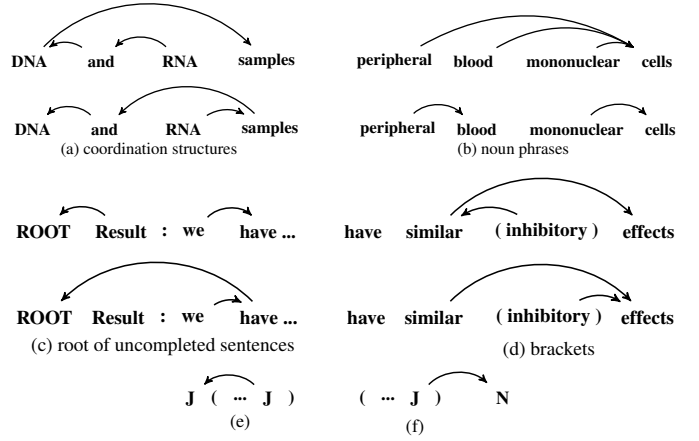
Figure 2: Unreliable arcs outputted by WSJ model
