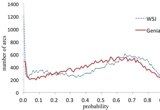
Figure 1: Probabilities of gold arcs assigned by different models
