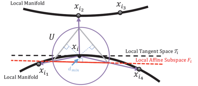
Figure 1: The best fitted local affine subspace \mathbf{F}_i (red dashed line) consists of two local directions \frac{\mathbf{x}_{i1} - \mathbf{x}_i}{\|\mathbf{x}_{i1} - \mathbf{x}_i\|} and \frac{\mathbf{x}_{i4} - \mathbf{x}_i}{\|\mathbf{x}_{i4} - \mathbf{x}_i\|} , and holds the minimal distance to \mathbf{x}_i .
