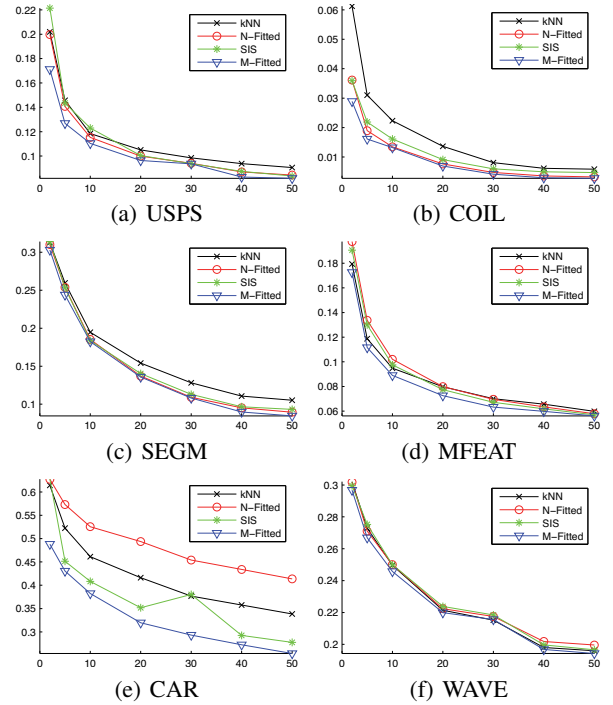
Figure 4: Average error rate vs. l for GFHF+CMN.
