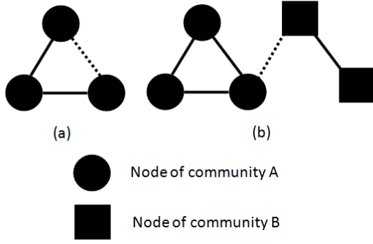
Figure 3: Two situations of a new edge link two existing nodes. (a)Nodes belong to a same community; (b)Nodes belong to different communities.
