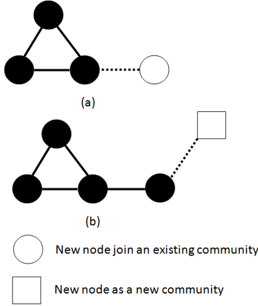
Figure 2: Split mechanism: (a) A new node attaches to an existing node with degree two, it join the same community of the existing node; (b) Another new node attaches to the previous new node with degree one, it split to a new community.
