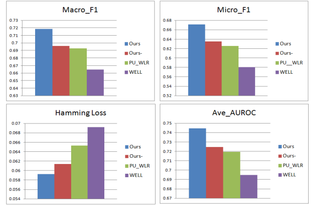
Figure 1: Performance of the proposed method in comparison with the state-of-the-art on MSRC image dataset. The dimension of the learned embedding is set r=64 .
