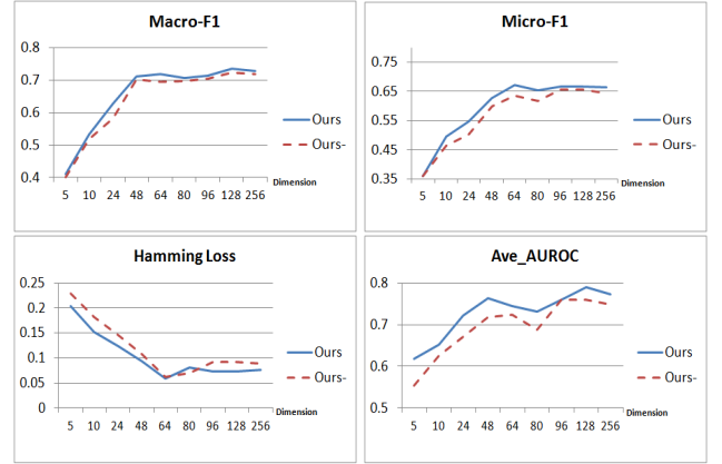
Figure 2: Performance of the proposed method ' ours ' and the degenerated version ' ours -' vs. the dimensions of embedding space on MSRC image dataset.
