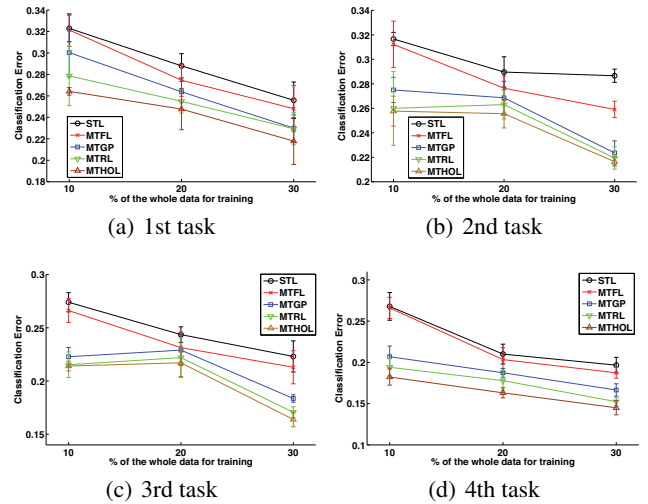
Figure 1: Performance of STL, MTFL, MTGP, MTRL and MTHOL on each task of the multi-domain sentiment application when the training set size is varied.
