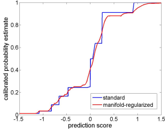
Figure 1: Calibration curve obtained on the ijcn1 data set. The abscissa is the classifier score and the ordinate is the calibrated probability produced by isotonic regression with (red) and without manifold regularization (blue).
