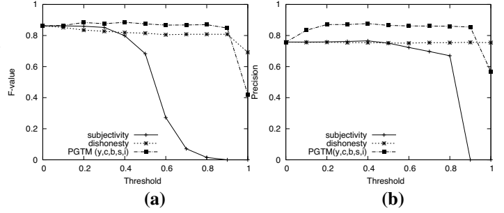
Figure 4: Model Effectiveness (Subjectivity vs. Dishonesty)
