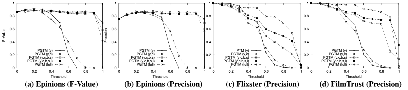
Figure 3: Model Effectiveness by Varying the Trust Threshold
