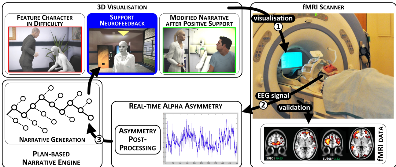
Figure 1: System Overview and Experimental Setting: (1) the user watches the narrative generated in real-time from inside an MRI scanner; (2) BCI input is interpreted in terms of empathy towards the feature character; (3) successful neurofeedback influences the narrative, improving the character’s situation.
