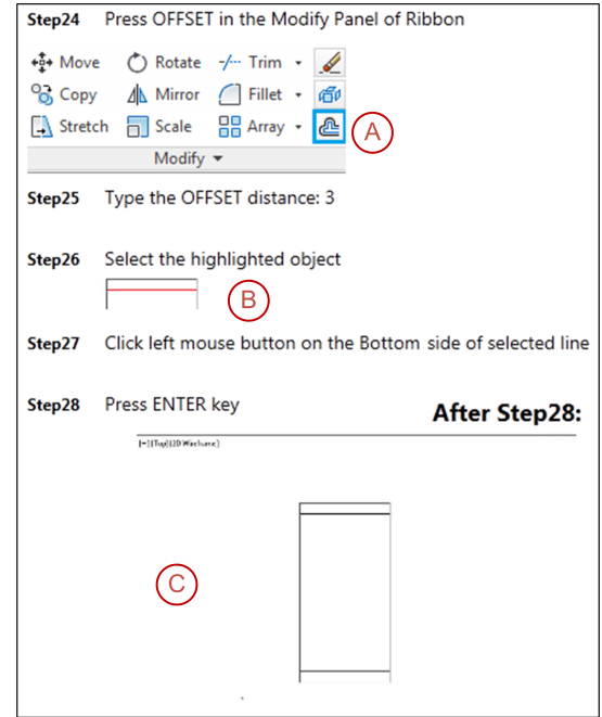
Figure 2: Generated tutorial at Figure 1(4)
