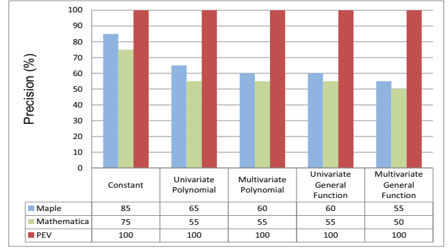
Figure 4: Performance Results based on Precision
