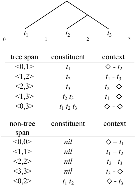
Figure 1. Illustration of constituents and contexts over a sentence “ t_1 t_2 t_3 ”
