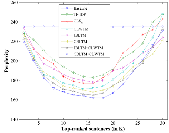
Figure 2: English reference translations based perplexity of adapted LMs vs. the size of selected training data with different approaches on the tuning set.
