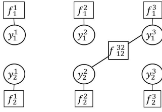
Figure 1: A factor graph for answer extraction. Circle nodes represent random variables for denoting word labels; rectangle nodes indicate factors connected to a single variable or two variables across different passages
