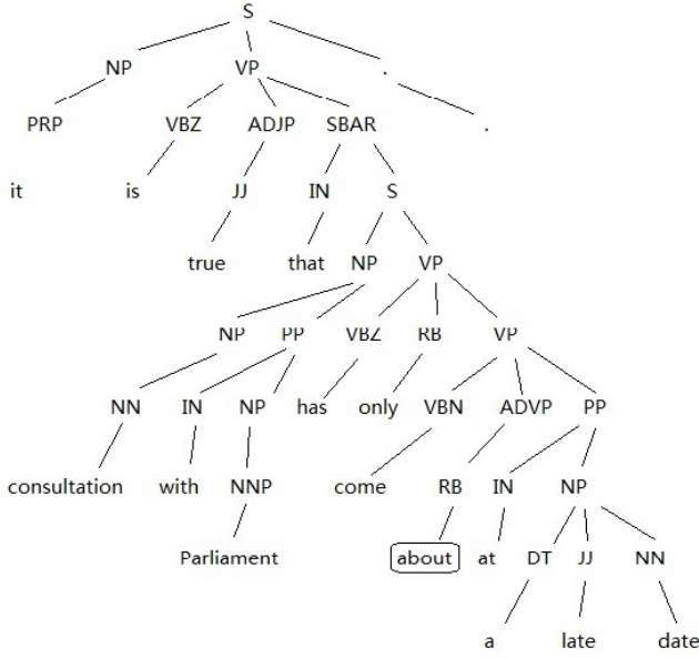
Figure 3: An example of constituency-based parse trees.
