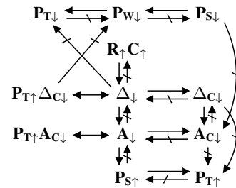
Figure 2: Relationships for \mathbf{M}_\uparrow transformations.
