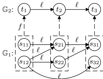
Figure 3: P_{S\uparrow} but not A_\downarrow .
