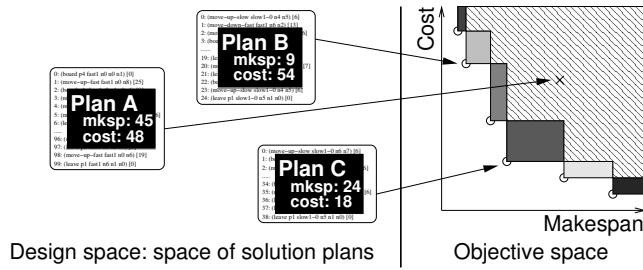
Figure 1: Design and objective spaces for a two-objectives planning problem. The hatched+grey area contains all images of possible solutions plans; this area defines the hypervolume of the set of circles, and the hypervolume contribution of each point is the grey area of the corresponding small rectangle (see Section 3). Circles are Pareto-optimal (non-dominated) solutions, aka the Pareto front of the problem at hand.
