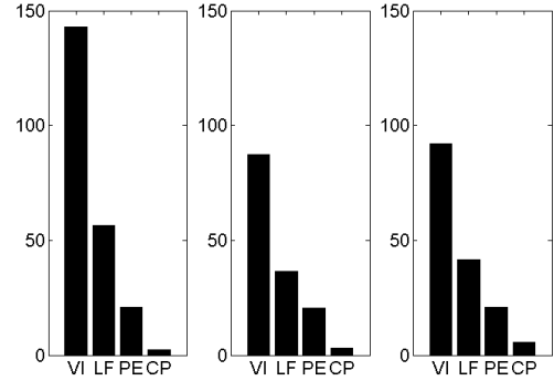
Figure 2: Relative difference in total cost with respect to the lower bound for the racetrack domain
