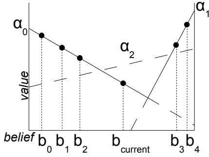
Figure 1: Point based value iteration. b_{current} is a belief state with low value according to the known \alpha_0 and \alpha_1 but where a better \alpha -vector \alpha_2 may be found.
