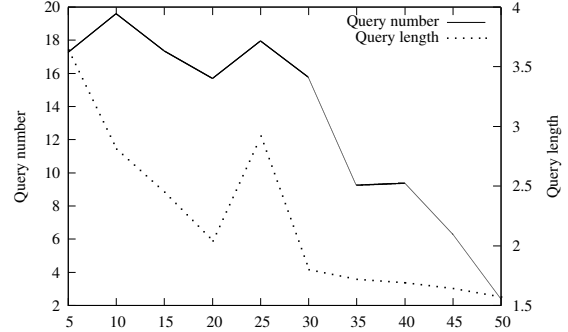
Figure 2: Results as a function of m with n = 50, k = 10 .
