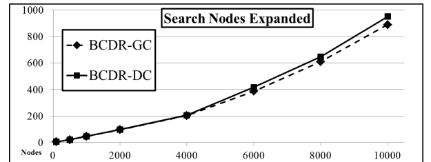
Figure 5: Performance of BCDR-GC and BCDR-DC on problems of low relaxation costs
