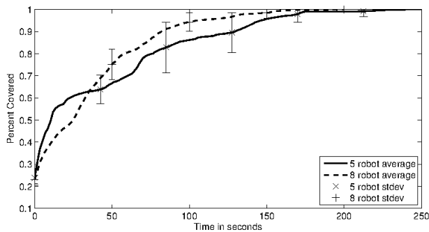
Figure 4: Average percent of the environment covered over time for five and eight robots (ten runs each). Error bars show standard deviation at that time point.
