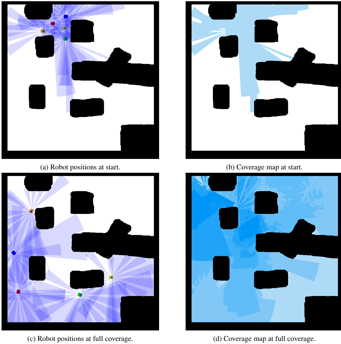
Figure 3: Five robots in the cave environment.
