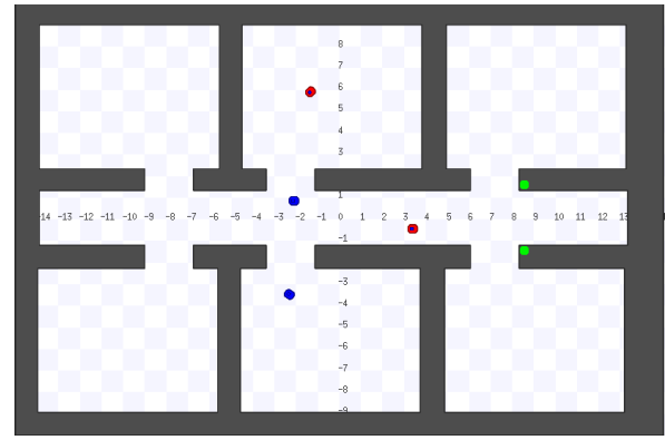
Figure 2: A simple environment with exploration partially completed. The robots (red and blue) are moving right to left, and have dropped two beacons (green) so far.
