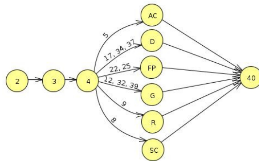
Figure 1: A finite state machine for Alg. 1. Numbers refer to lines in Alg. 1 and letters are behavior initials.
