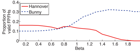
Figure 3: Effect of \beta on the proportion of the unique FPFHs that led to valid matches for the Hannover and Bunny datasets.
