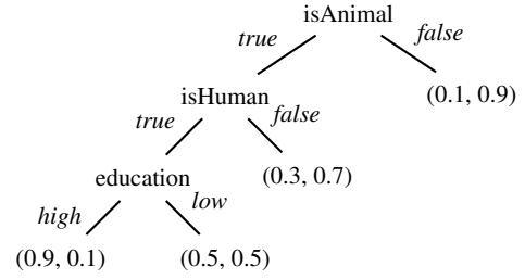
Figure 1: A tree-structured representation for P(\text{causeDamage} \mid \text{isAnimal}, \text{isHuman}, \text{education}) . The leaf nodes specify probability distributions over \{\text{true}, \text{false}\} for causeDamage .
