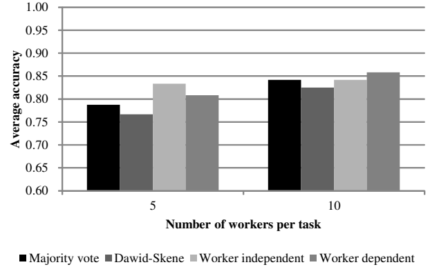
Figure 5: Results for binary question answering
