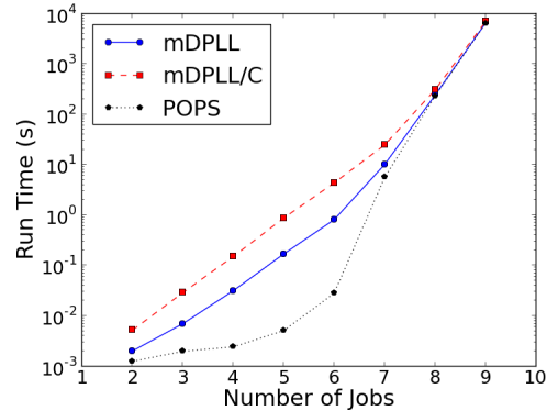
Figure 2: Log runtimes for #SAT job shop scheduling instances with 2 machines, 2 bits of uncertainty and 8 time steps.
