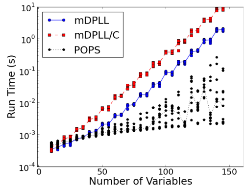
Figure 4: Log runtimes for random 3 \# SAT instances on graphs with a clause ratio of 2.5 and 10% \Sigma -variables. Medians are plotted as a trend line, and individual instances are plotted as points.
