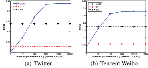
Figure 6: Comparison of Recall@20 varying the scale of the social parameters e , f and g .
