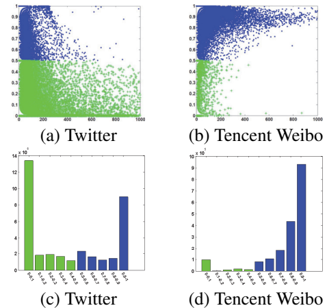
Figure 1: For (a)(c), 200,000 users were sampled, each point (x,y) represents a general user, where x is the number of followees and y is the percentage of celebrities in this user’s followees. For (b)(d), all users are used, the height of each bar represents the number of users with corresponding percentage of celebrities in their followees.
