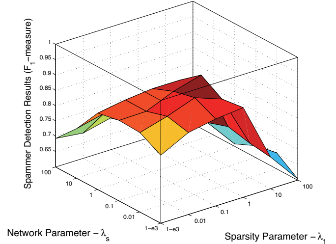
Figure 2: Impact of the Sparsity Parameter ( \lambda_1 ) and the Network Parameter ( \lambda_s )
