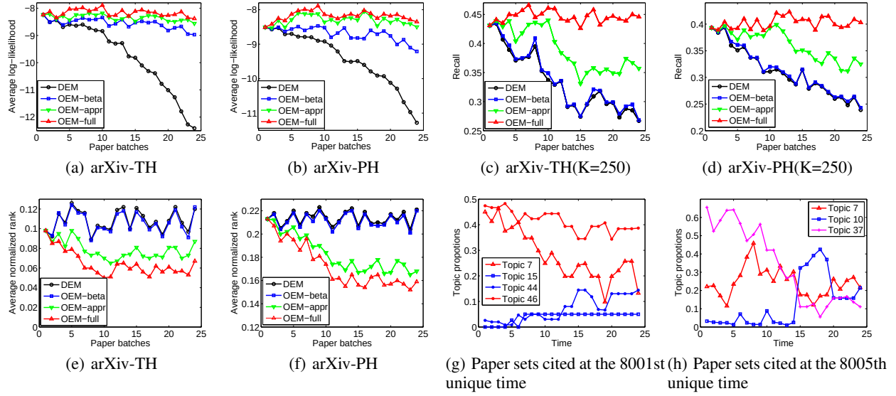
Figure 1: (a) and (b) are the average held-out log-likelihood of testing citation events. (c) and (d) are the recall of top-K recommendation lists. (e) and (f) are the average held-out normalized ranks of testing citation events. Since all models have the same initial parameters after the building and training phases, all models have the same performance on the first testing batch, which can be seen from (a) to (f). (g) and (h) are the topic evolution of sets of papers cited at the 8001st and 8005th unique time. To avoid clutter, we only show the topics with the largest proportions (top topics).
