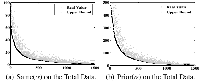
Figure 3: An illustration of upper bound.
